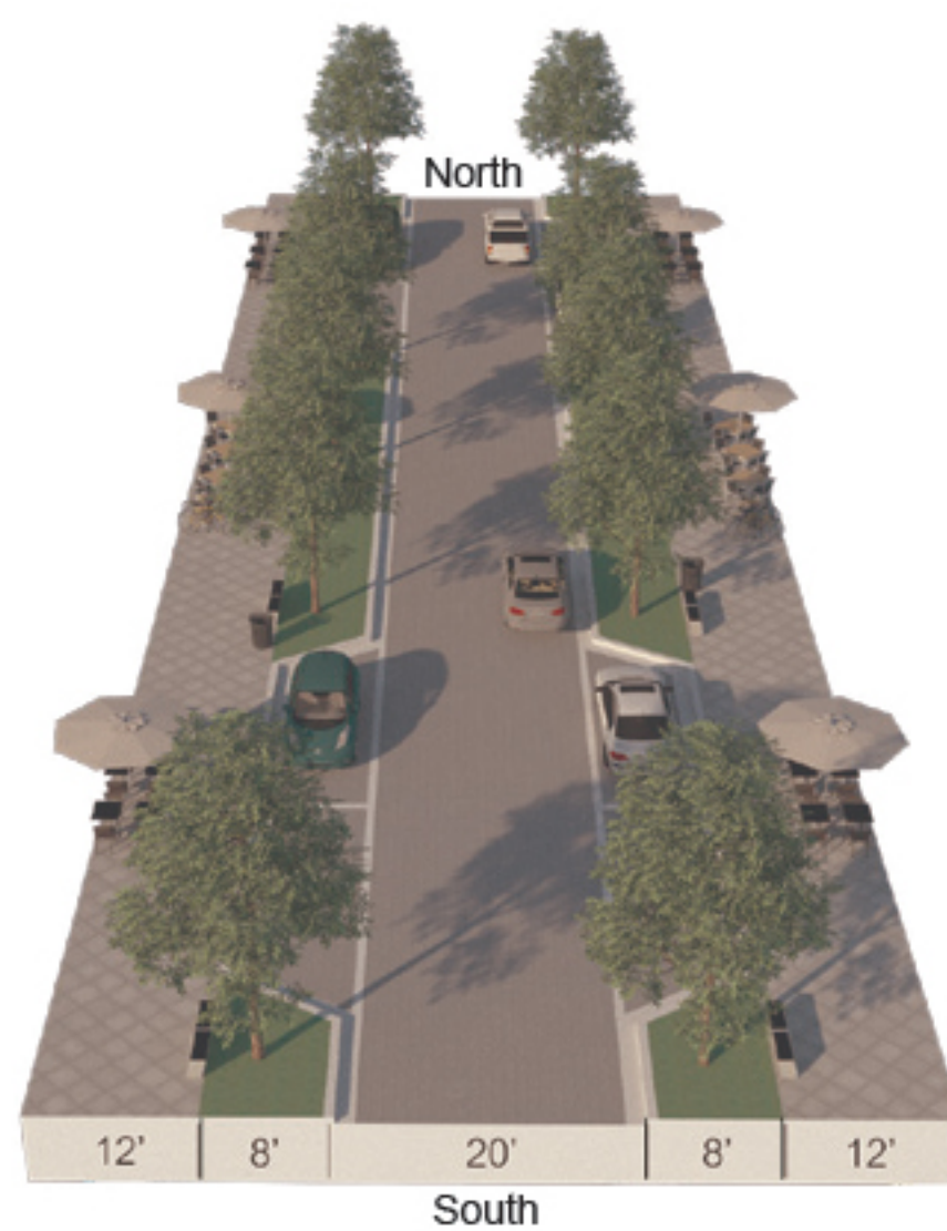
Concept 1a Two-Way Street On-Street Parallel Parking Street Trees Wider Sidewalks Curbed Design
